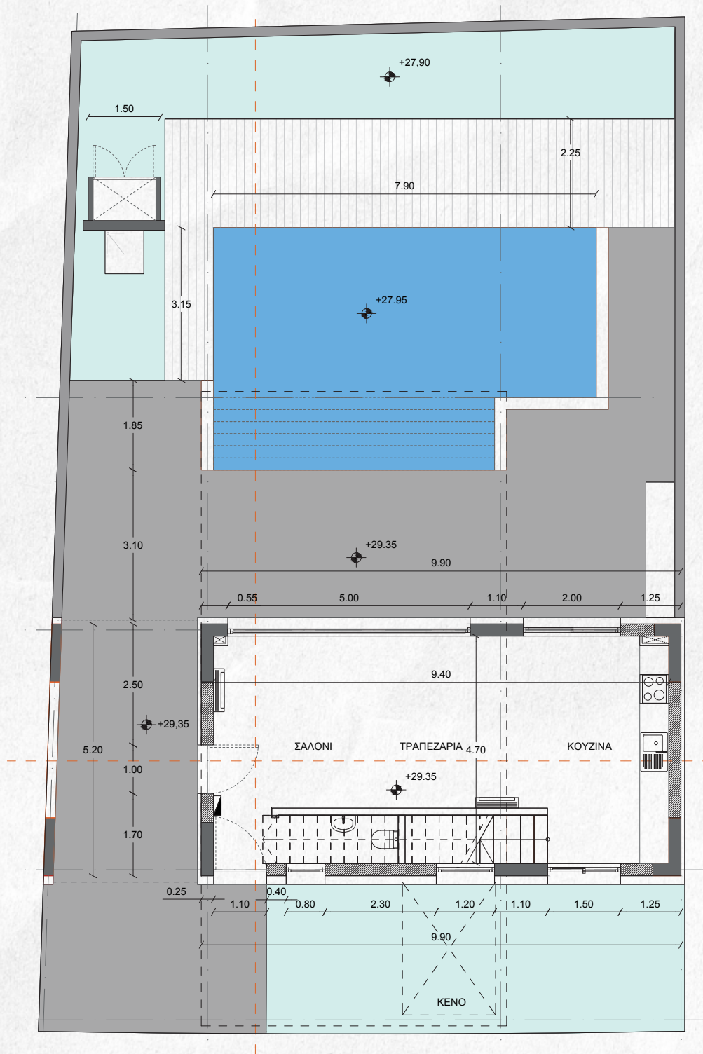
GROUND FLOOR
