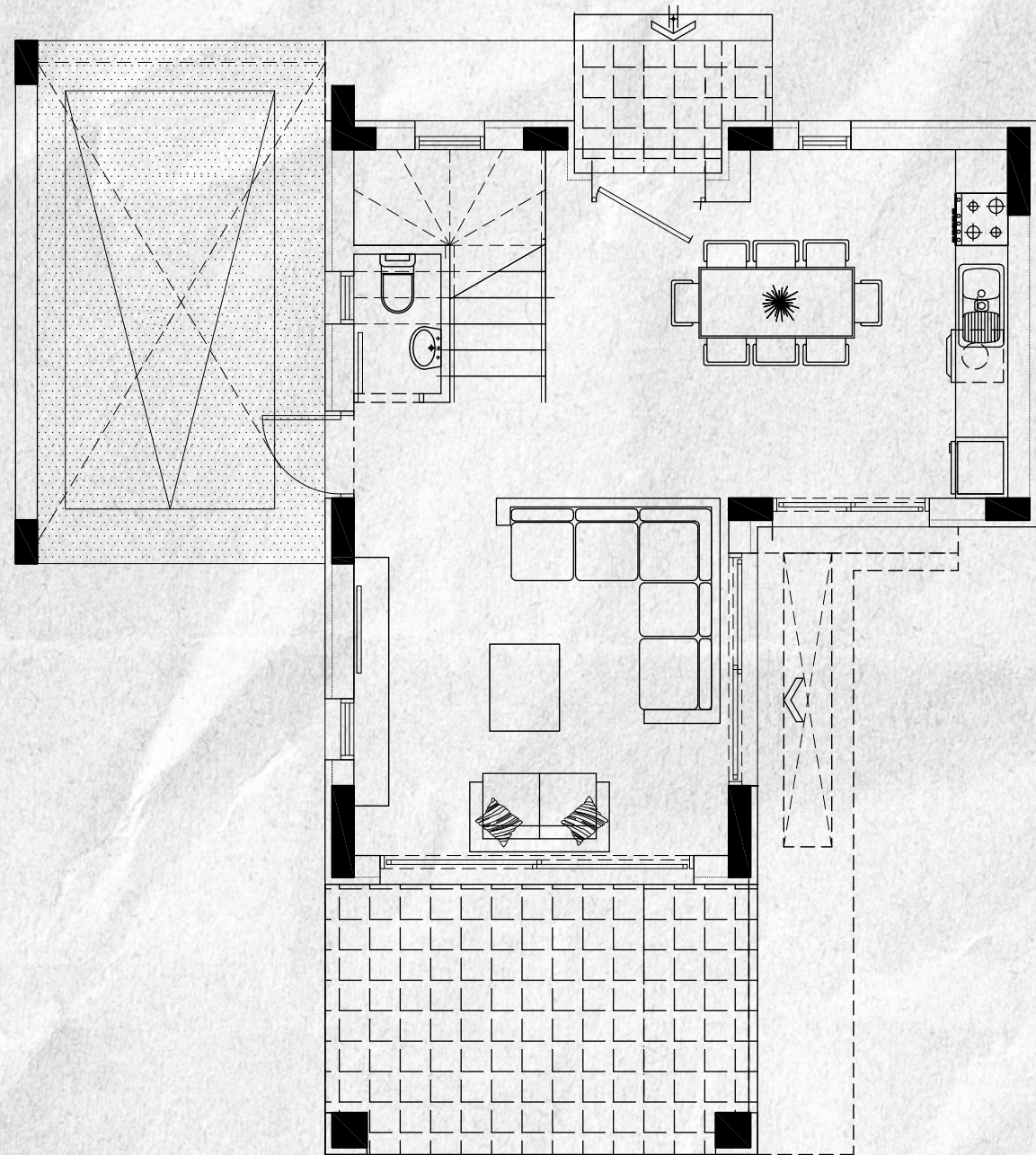
GROUND FLOOR
